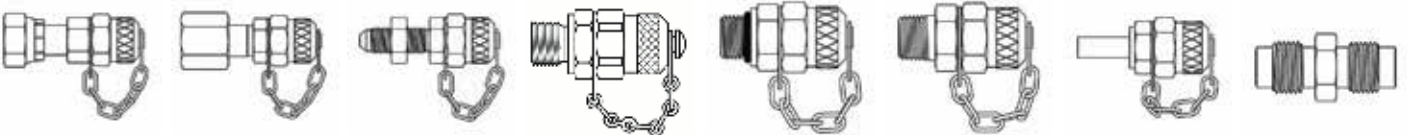
TPFF ORFS Swivel to Test Point with Seal Retainer TPFJ JIC Swivel to Test Point TPBH JIC to Test Point Bulkhead with Locknut TPM Metric to Test Point TPO O-Ring to Test Point TPP Pipe to Test Point TPSP Metric Standpipe to Test Point TPU-U Test Point to Test Point (No Check Valve)
